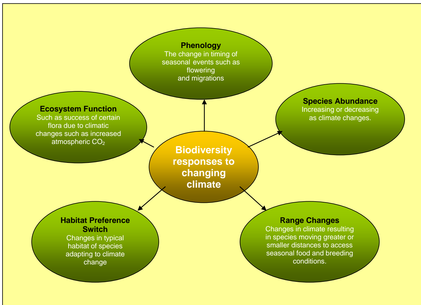
Figure 3 Specific responses by biodiversity and ecosystems to climate change
